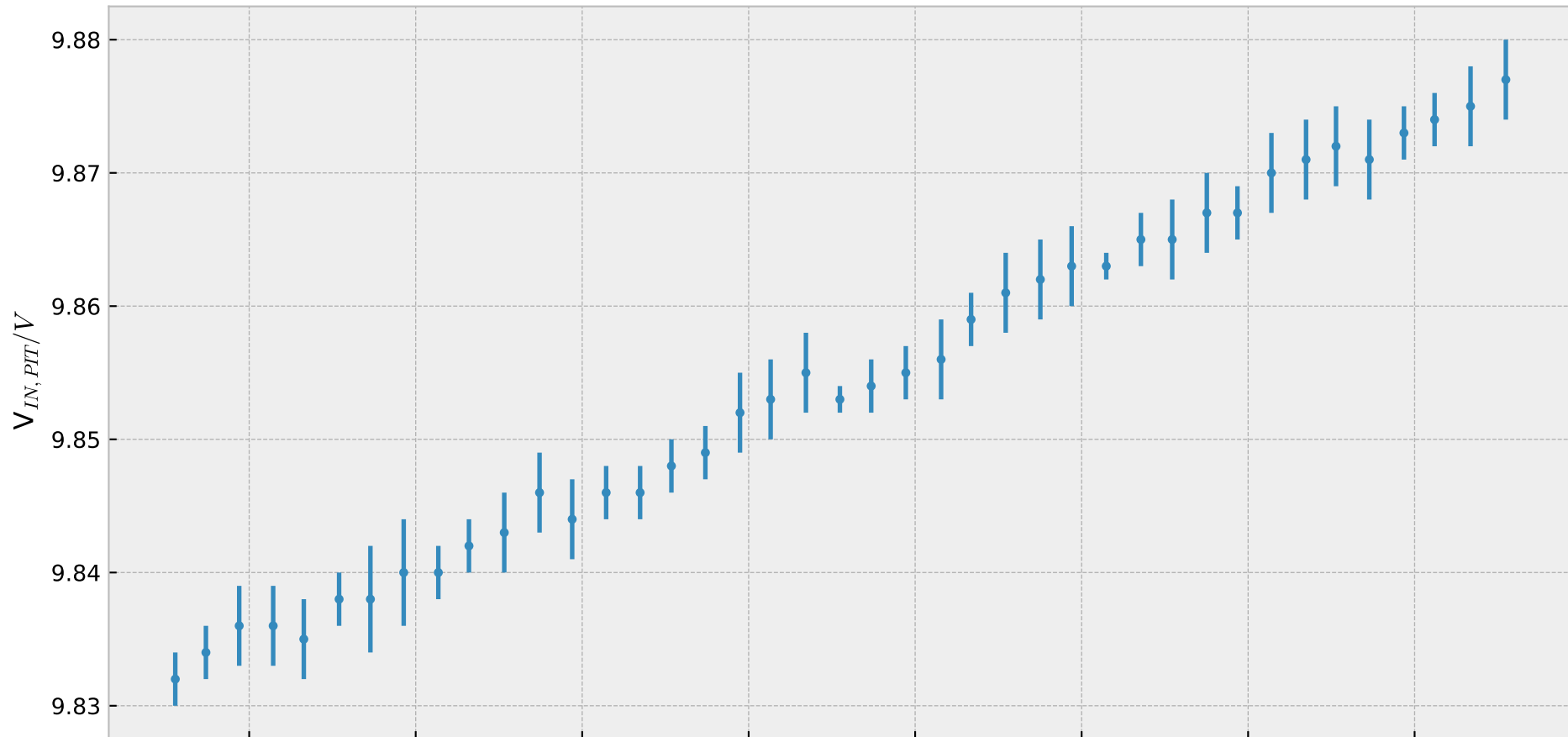
PowerIt ADC Calibration: 48V Input
