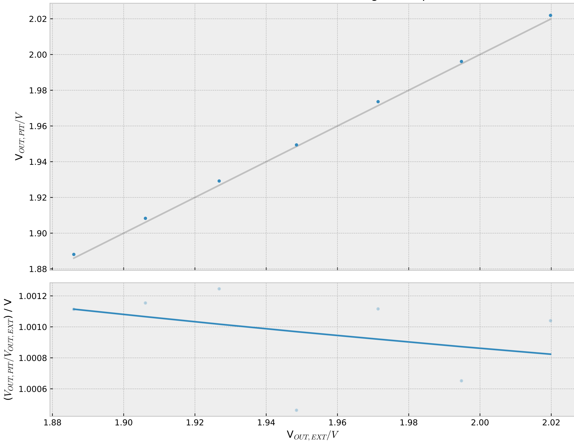
PowerIt ADC Calibration: 1V8 Digital Output
