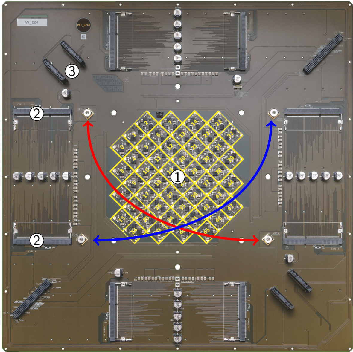
Figure 2.7.: A photograph of the top of the MainPCB (courtesy of Maurice Güttler [?]). The board has a length and width of 43cm. Visible in the center are the PowerFETs (Field Effect Transistors) (1) which switch the power supply of each reticle. These are controlled via the CURE boards (2). In yellow the corresponding Reticle and its position is marked. All 48 Reticles are shown. A single reticle has a width of 20.0482 mm and height of 20.145 mm, with additional space in between reticles of 420 \mu\text{m} horizontally and 250 \mu\text{m} vertically [?]. The top-left and bottom right corner connectors (3) are for the AnaB boards. The main supply voltages V_{DDA} (red) and V_{DDDD} (blue) are generated on the PowerIt and inserted at the marked screw connections.
