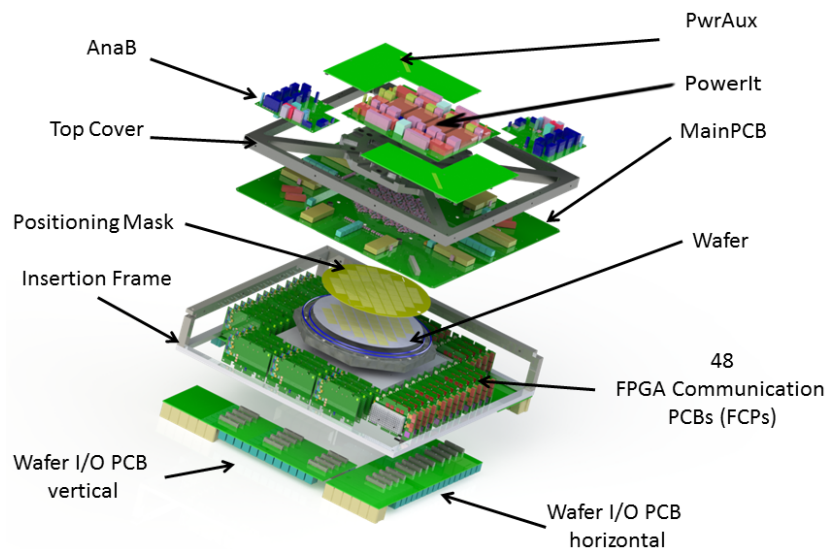
Figure 1.1.: The BrainScaleS wafer-scale hardware system, marked are the main components comprising a single wafer system. [?]
