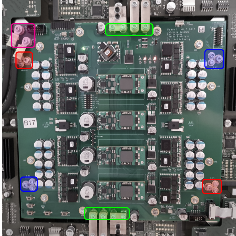
Figure 1.2.: Photograph of the PowerIt boards top view. Its receiving 48 V as input (magenta) and outputting 9.6 V (green) as well as 1.8 V (analog: red, digital: blue)
